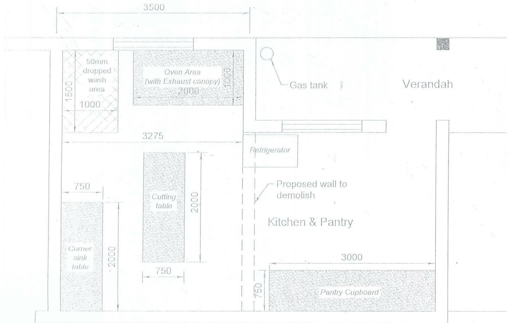
Revised kitchen layout Guest House
