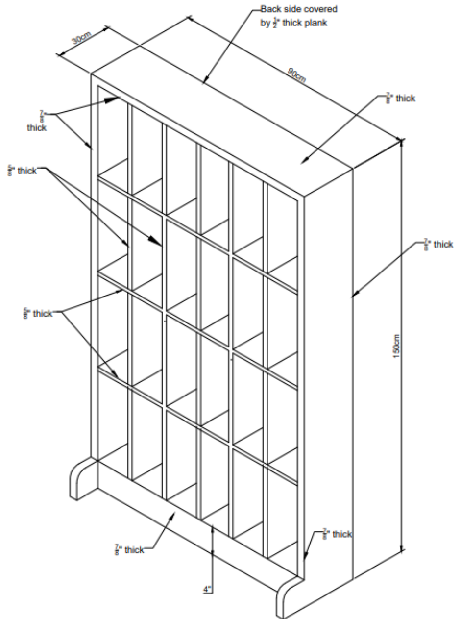
Pigeon Hole Rack
