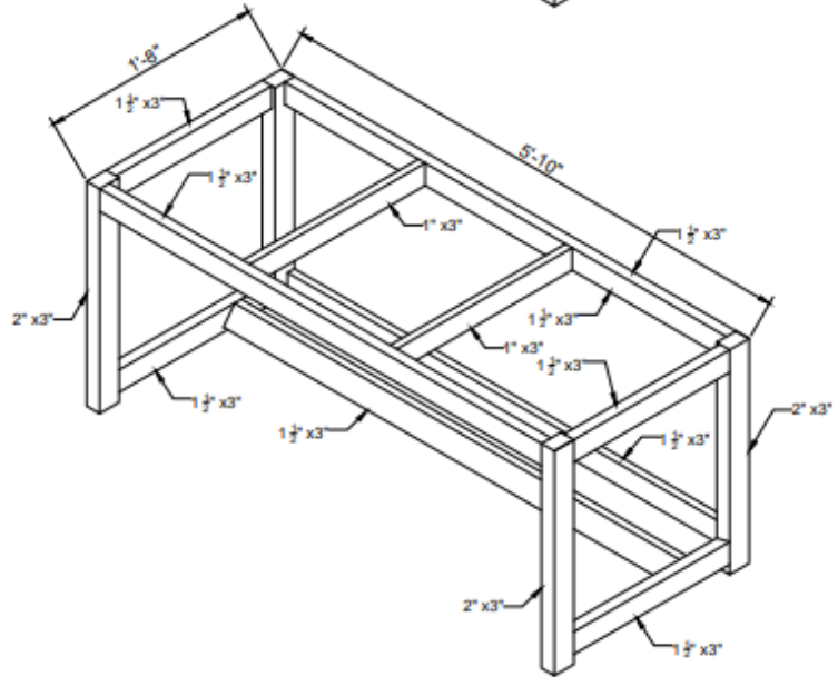
Wooden Multi Purpose Table for Canteen
