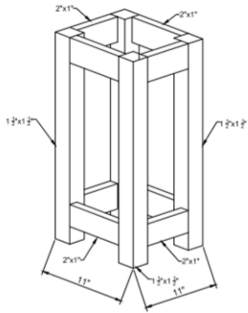
Wooden Stool For Laboratory
