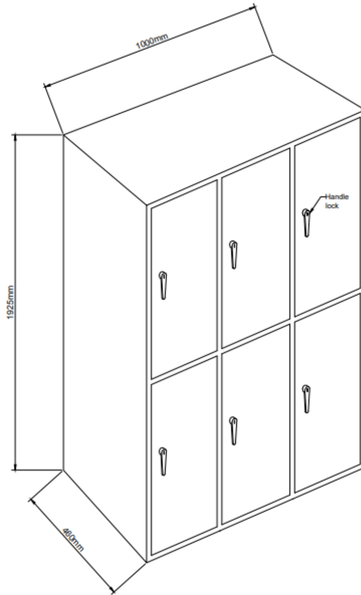
Steel Workmen Locker (6 Units)
